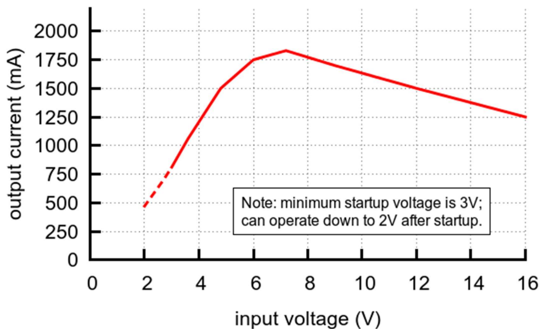
Maximum Continuous Output Current
